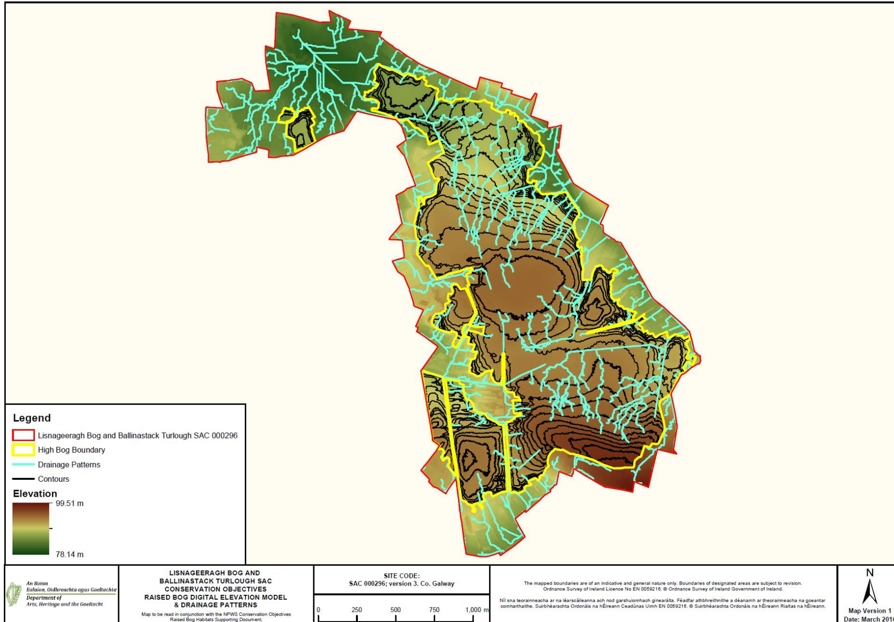
Map 3: Digital elevation model and drainage patterns at Lisnageeragh Bog.
