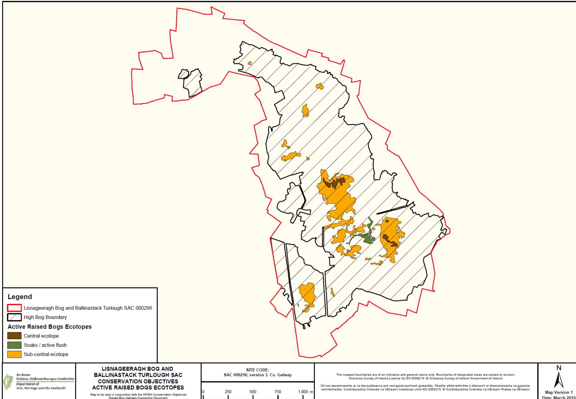
Map 2: Distribution of raised bog ecotopes on Lisnageeragh Bog.
