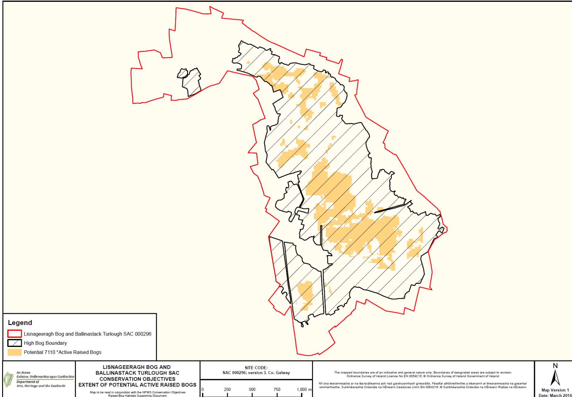
Map 1: Extent of potential active raised bog on Lisnageeragh Bog.
